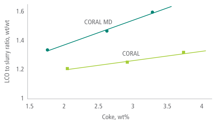
Figure 2: CORAL MD enhances the LCO/slurry ratio.
